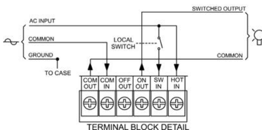
SWITCHED LOADS
