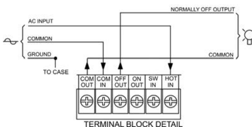
SWITCHED LOADS
